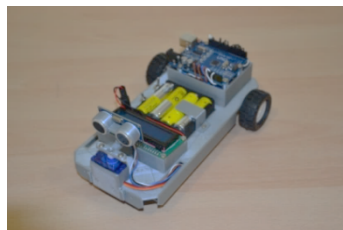
ROBOT INVENTUS (fabrication C.T.A.)
